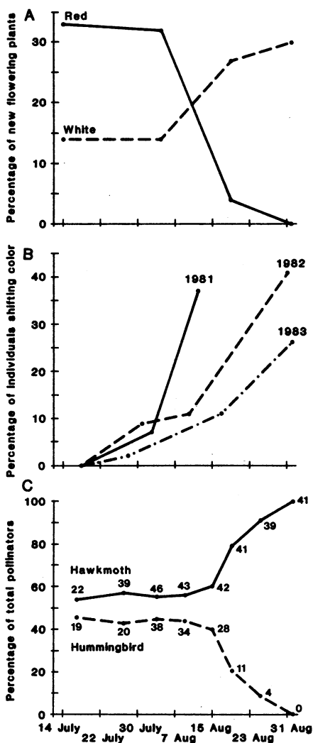
Fig. 1. Shifts in corolla color by populations (A) and individuals (B) of scarlet gilia in relation to pollinator abundance (C). (A) Plants initiating flowering early in the season were darker in color, whereas plants initiating flowering later produced lighter corollas. Pink individuals (not shown) displayed flower patterns intermediate to those of red and white individuals. (B) Individual plants shifted color during the flowering season. Three years of data are shown. Sample sizes for 1981, 1982, and 1983 are 482, 1282, and 2463 plants, respectively. (C) The two primary pollinators of I. aggregata changed in abundance during the flowering season. Numbers adjacent to points represent the number of pollinators observed on a particular date. Data shown are for 1983. Pollinator abundance data collected in 1982 also correspond with floral shifts.
