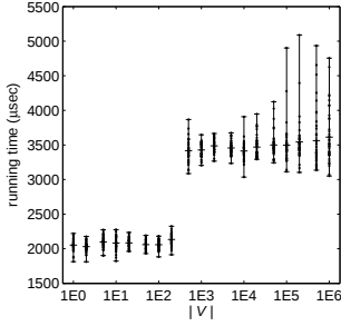
Figure 4. Database view updates.
