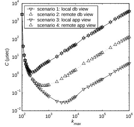
Figure 6. Expected maintenance cost.
