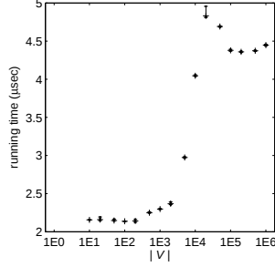
Figure 5. Application view updates.
