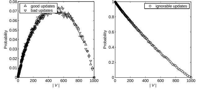
Figure 1. Results from the first simulation.
