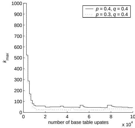
Figure 8. Behavior of the adaptive algorithm.
