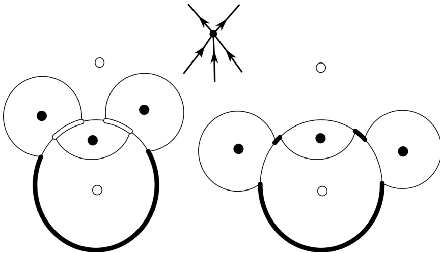
FIGURE 2. Singular sets and trajectories of clean quadratic differentials on \mathbb{CP}^1 with 5 poles of order 2, and 6 simple zeros each. The residues of \sqrt{\Psi} at the poles (equal to the widths of the circle domains centered at these poles) are the same on the left and on the right. Yet the potential on the left has negative components of \mu_F ; the one on the right is positive. The Reeb graph is sketched on the top. (We keep the convention that positive masses are shown as solid lines or dots; negative, - as hollow ones.)
