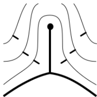
FIGURE 3. Positivity forces the orientation of the potential function near a simple pole of \Psi .
