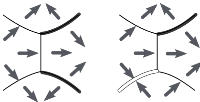
FIGURE 1. The figure showing how the orientation of the Reeb graph affects the positivity on a component of K_\Psi : on the left display, all edges of the fat graph component have the Reeb graph orientation pointing toward them, or “through” them; on the right display, the SW edge has both adjacent edges of the Reeb graph outgoing, resulting in locally negative mass. (Positive charges are shown as fat solid lines, negative, - as fat hollow line.)
