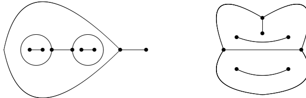
Figure 5. K_\Psi admitting and not admitting a positive measure
