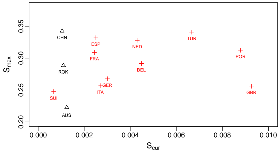
S_{\max} vs S_{\text{cur}} (confirmed cases) in the dashed frame
