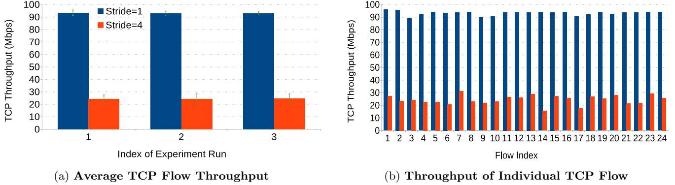
Figure 7: Mininet Emulation Results: ECMP Limitation in a Fat-tree-based Data Center Network with 100 Mbps Link Bandwidth
