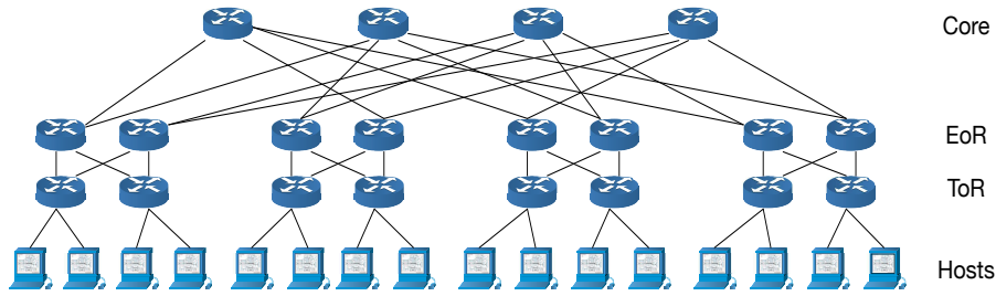
Figure 6: A Data Center Network with a Degree-4 Fat Tree Topology
