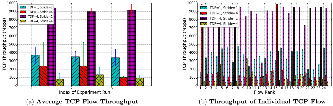
Figure 8: Mininet Emulation Results with Virtual Time: ECMP Limitation in a Fat-tree-based Data Center Network with 10 Gbps Link Bandwidth
