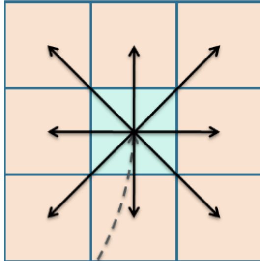
Figure 1: Simple A* [4]
