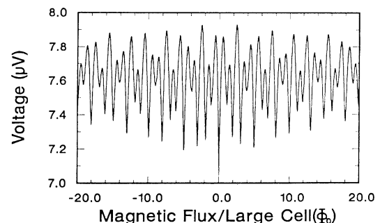
FIG. 3. Voltage vs magnetic flux/large cell for a bias current of 70 \mu m A and a temperature of 1.12 K.
