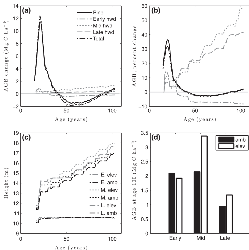
Fig. 3. Model predictions of change in aboveground biomass and height under eCO 2 by PFT: (a) absolute differences: change = elevated AGB - ambient AGB for each year and PFT; (b) percent change by PFT, change = [(elevated AGB - ambient AGB) / ambient AGB]; (c) height of tallest hardwood cohort by PFT; (d) hardwood AGB after 100 years of regrowth.
